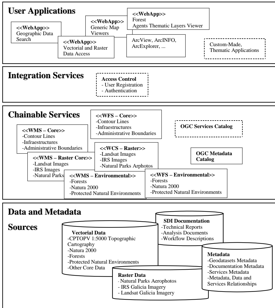
Fig. 1 Service-oriented view
